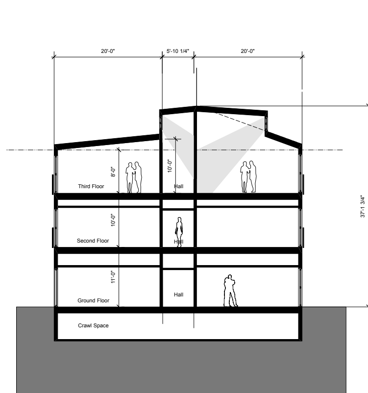
Building Section @ Dormer Windows
