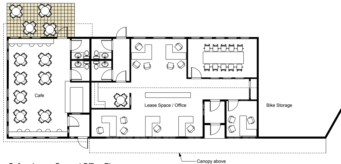
Cafe + Lease Space / Office Plan
