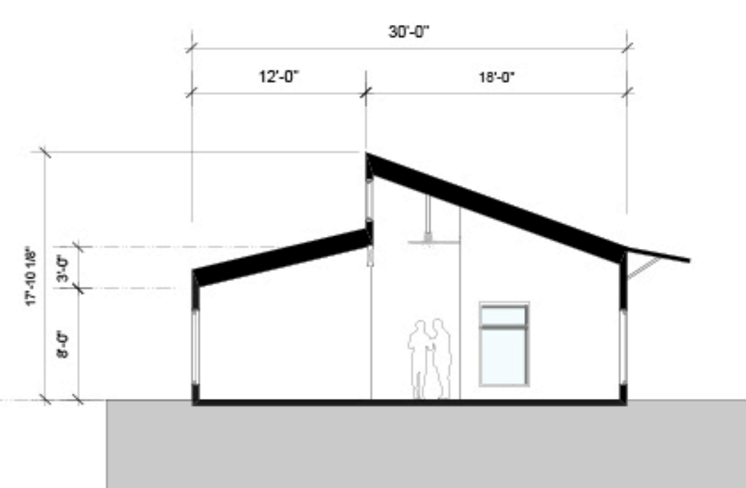
Lease Space Section
