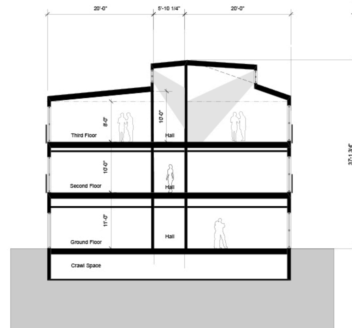
Building Section @ Dormer Windows
