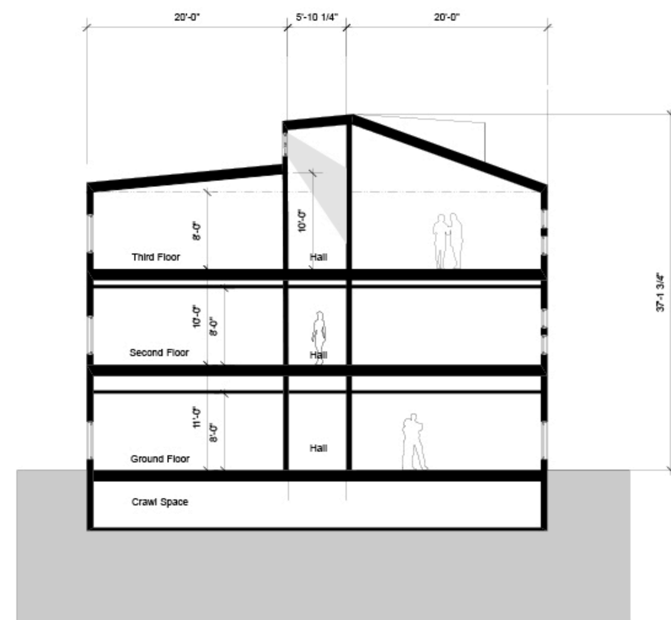
Building Section
